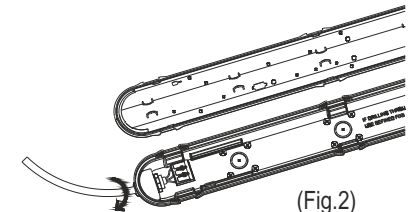
(Fig.2) Route mains supply cable into the base and wire it to the terminal block of the light fitting. Ensure L, N and Earth are wired correctly.
