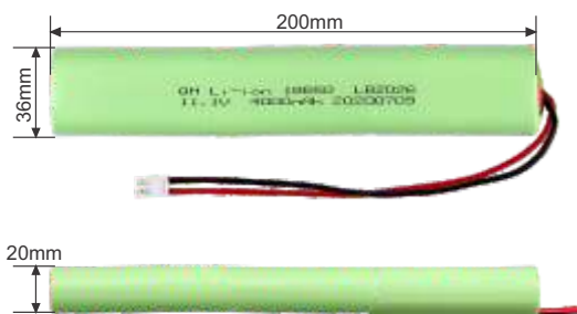
Fig. 2 Battery Dimensions
