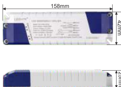
Fig. 1 Inverter Dimensions
